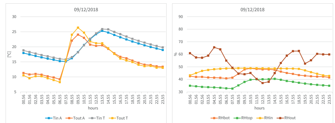
Figure 219 / Comparison of temperatures measured inside and outside with Thermozig and Domino
