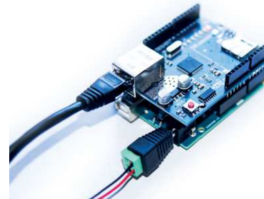
Figure 169 / Ethernet shield W5100 connected to Arduino™ Genuino101
