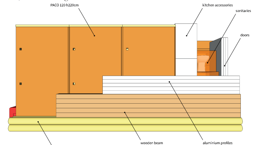
Figure 124 / ▼ Load design of Container ISO 20 ft - Left view
