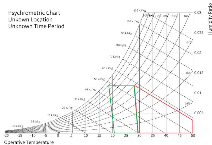
Figure 105 / Green: comfort polygon; red: CPZ for evaporative cooling
