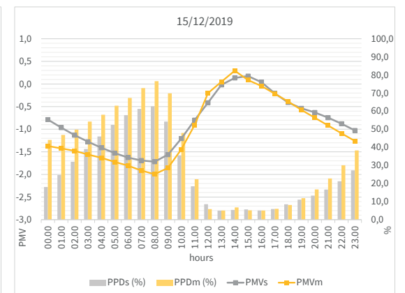
Figure 216 / Comparison of comfort indexes from measurement and simulation, PMV and PPD
