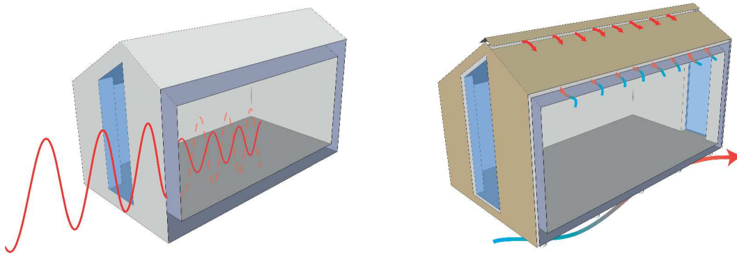
Figure 130 / ◀ Time lag and reduction of thermal wave due to thermal mass Figure 131 / ▶ Ventilated façade example of operation
