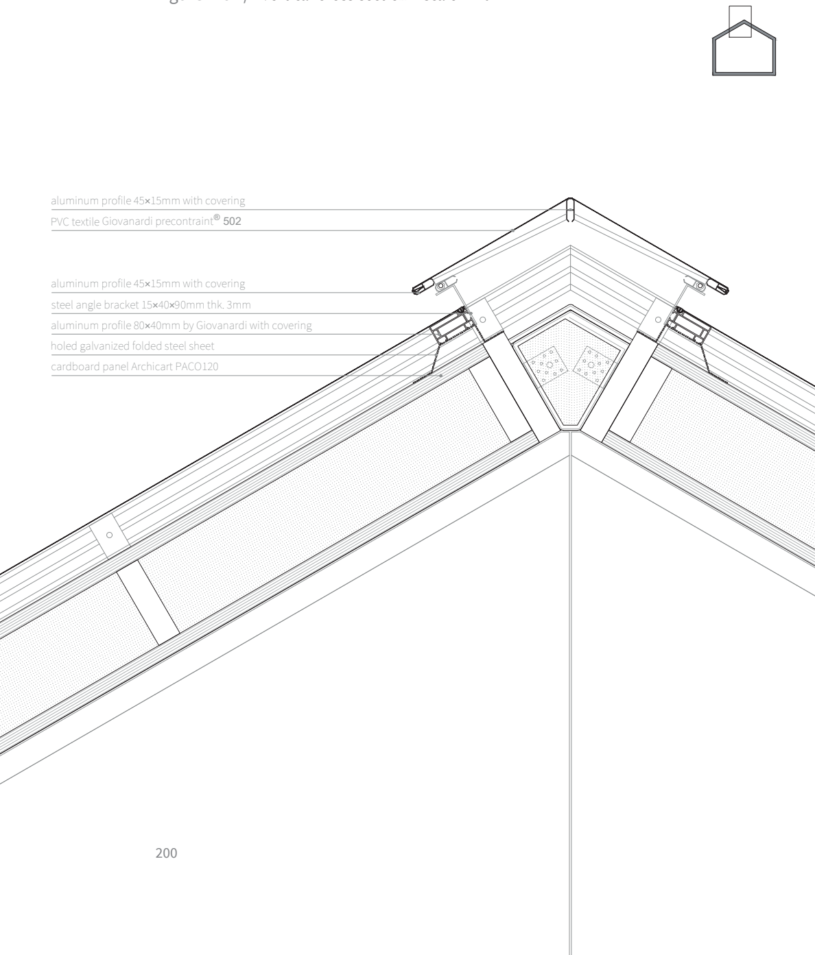
Figure 162 / Vertical cross section - scale 1:10
