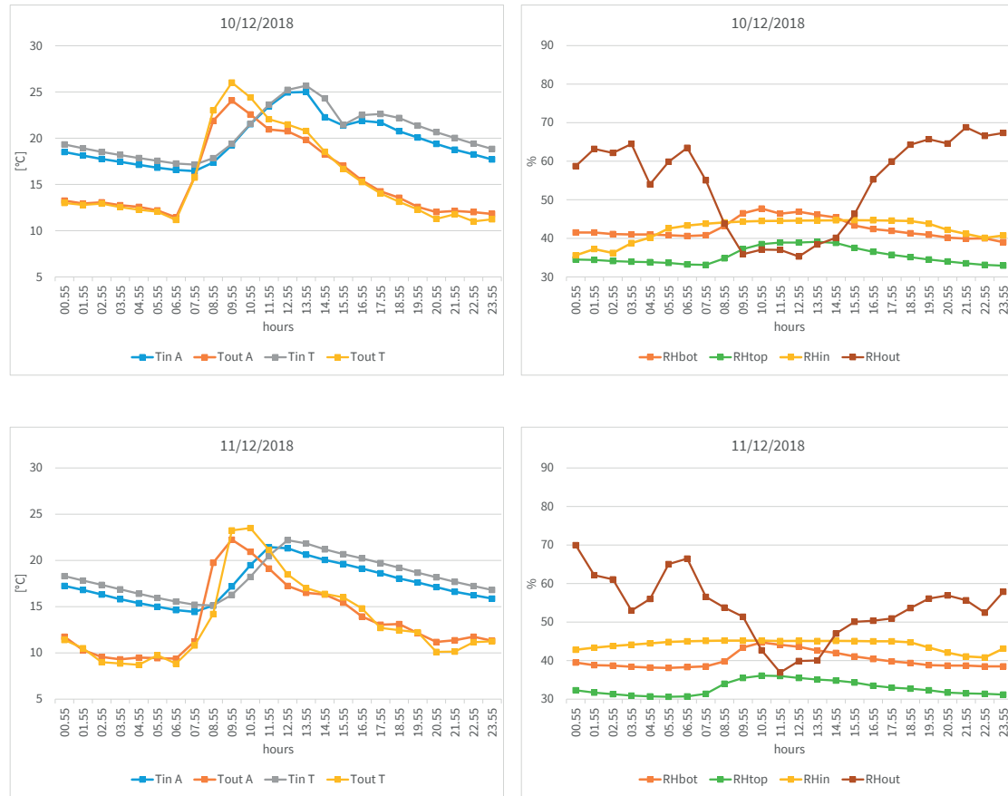
Figure 221 / Comparison of temperatures measured inside and outside with Thermozig and Domino
