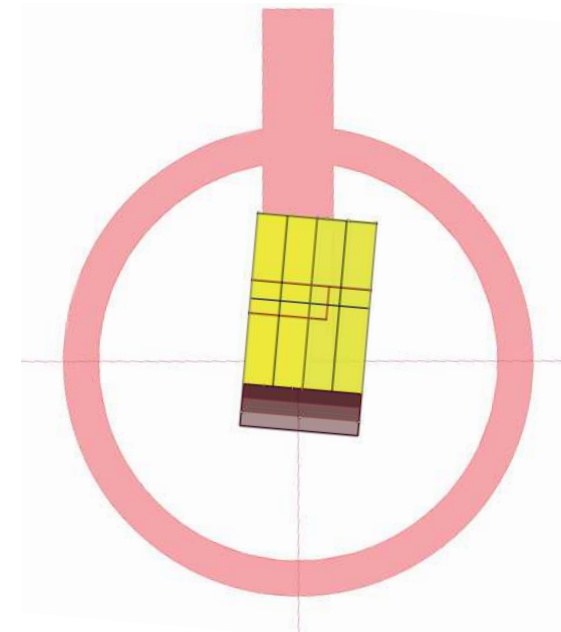
Figure 147 / ▲ Ladybug North
