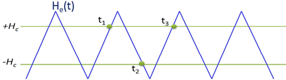
Fig. 1.6 – Triangular driving magnetic field.
