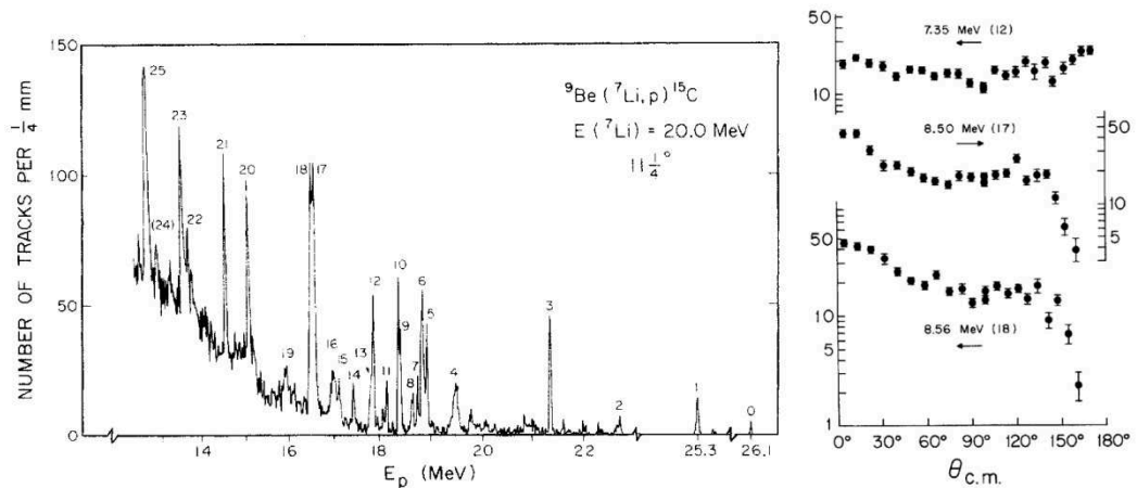
Fig. 4.12. Proton spectrum from the {}^9\text{Be}({}^7\text{Li},p){}^{15}\text{C} reaction at 20 MeV incident energy and \theta_{lab} = 11.25^\circ (left panel). The populated states indicated with the numbers are listed in Table 1 of ref. [104]. Angular distributions for the ^{15}\text{C} unbound states at E_x = 7.35 , 8.50 e 8.56 MeV [104] (right panel).
