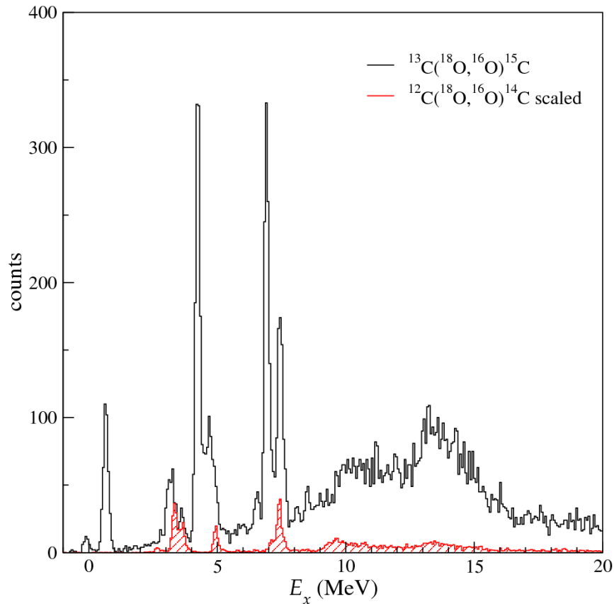
Fig. 6.19. Excitation energy spectrum of the ^{13}\text{C}(^{18}\text{O}, ^{16}\text{O})^{15}\text{C} reaction at 9.5^\circ < \theta_{lab} < 10.5^\circ . The red hatched histogram represents the normalized background of the ^{12}\text{C}(^{18}\text{O}, ^{16}\text{O})^{14}\text{C} reaction coming from ^{12}\text{C} impurities in the ^{13}\text{C} target.
