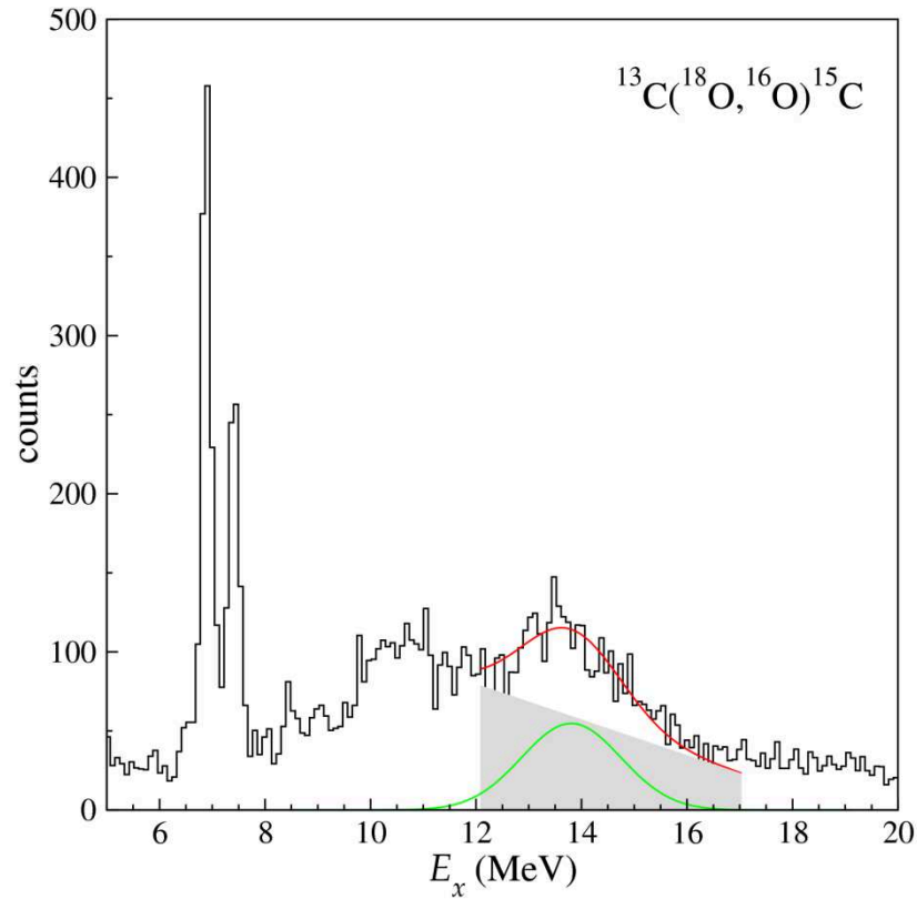
Fig. 6.30. Excitation energy spectra for the ^{13}\text{C}(^{18}\text{O},^{16}\text{O})^{15}\text{C} reaction at 9^\circ < \theta_{lab} < 10^\circ . The modeled 3-body continuum, the fitted peak and the sum of them are shown with the grey area, the green Gaussian and the red continuous line, respectively.
