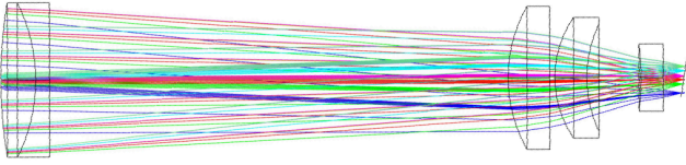
F . 4.— Camera layout. Spherical surfaces and standard glasses ensure high transmission and low-cost. Note the tilted focal plane to correct for axial chromatism.
