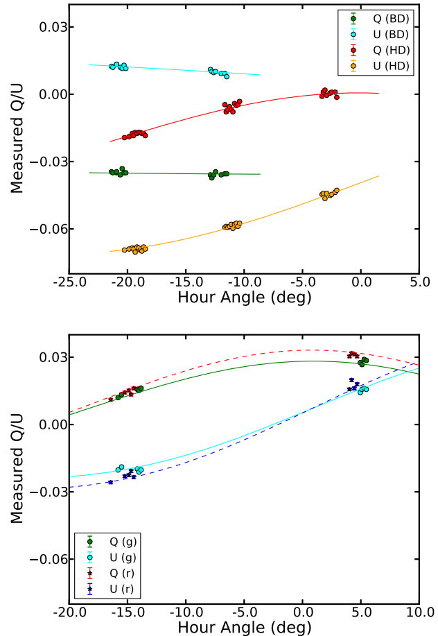
Fig. 8 Polarimetric standard star observations (BD +28 ^{\circ} 4211 and HD 204827) carried out on 2012 October 5 ( upper panel ) and (GD 319) on 2013 January 27 and 28 ( lower panel ). We show our best-fit model superposed on the measured instrumental polarizations. The wavelength dependence of the instrumental polarization in this limited range is also well reproduced by the model.
