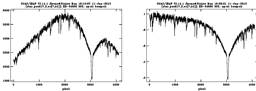
Figure C.4: Top panel: Extracted order of HARPS echellogram containing the H\alpha line. Bottom panel: Flux distribution after flat-fielding.
