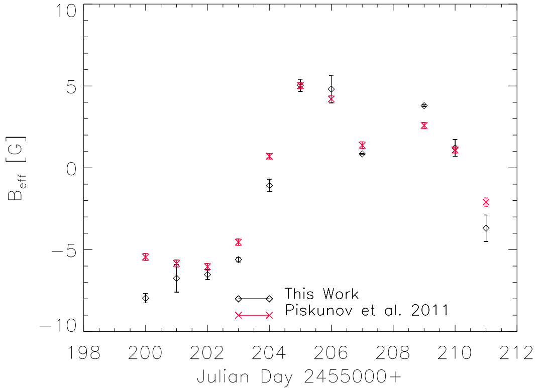
Figure 6.1: Comparison between the measurements of the effective magnetic field of \epsilon Eri observed with HARPSpol in 2010 (Kochukhov et al., 2011; Olander, 2013). The black points are obtained with our LSD code (black) and red points are the values obtained by Kochukhov et al. (2011).
